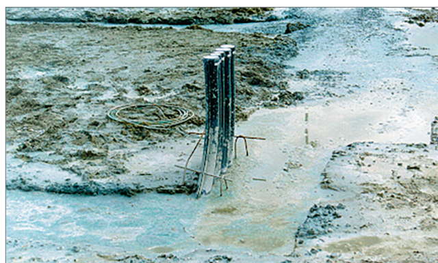
Energiebocht in fundering in volle grond
